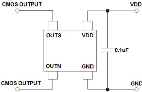
Figure 1, Typical Application Circuit of AS1827A
