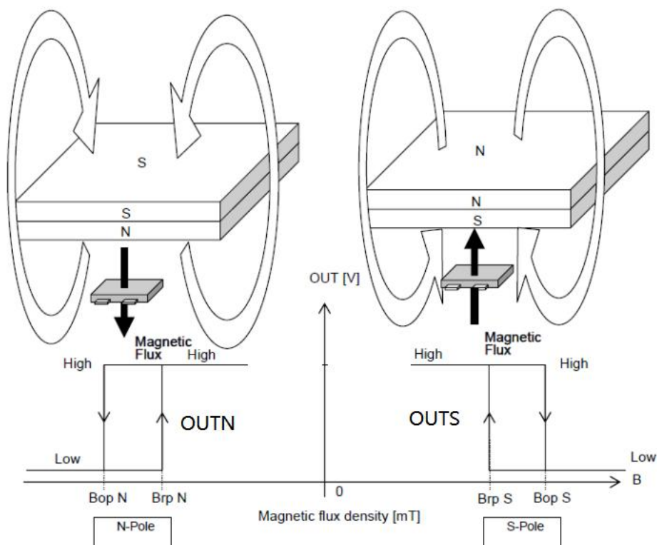
Fig 3, Magnetic Operation Characteristic of AS1827A
