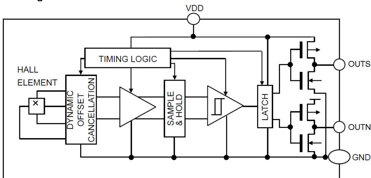
Figure 2, Block Diagram of AS1827A
